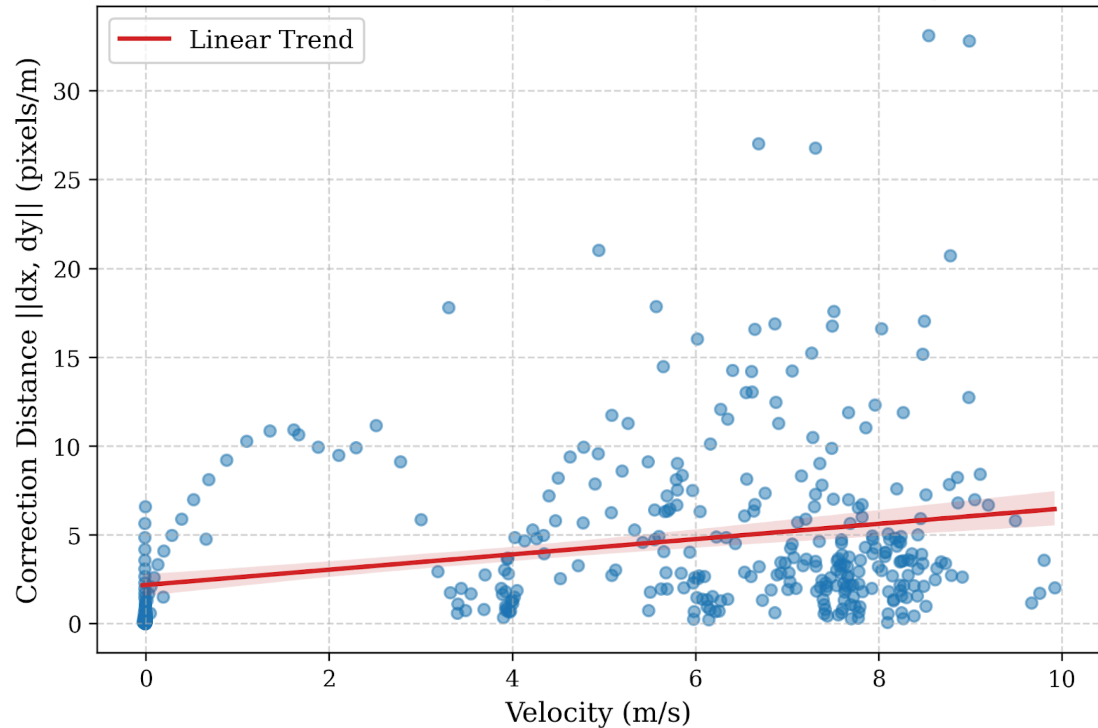
EKF Correction Magnitude vs. Vehicle Velocity
